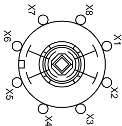
TYPICAL TERMINAL/ROTOR/STATOR ORIENTATION FOR ALL DECKS
